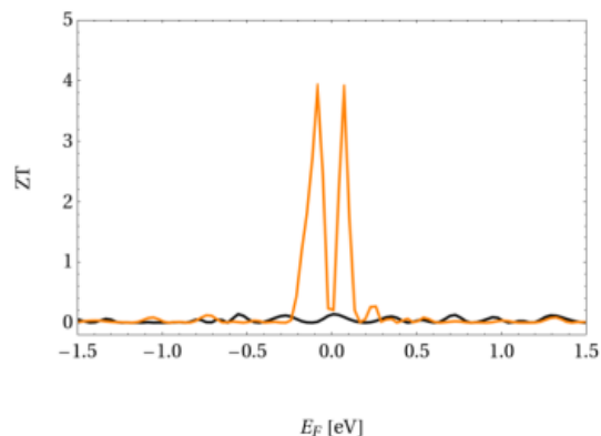
Fig 6: FOM as a function of Fermi Energy (EF) for a long-range hopping (LRH) magnetic helix in absence (shown by black line) and (b) presence (shown by orange curve) of light. Here, we set N = 10 and A_0 = 0.5 .
