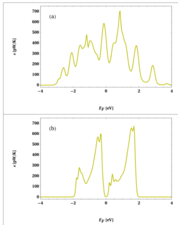
Fig 5: Thermal Conductance as a function of Fermi Energy ( E_F ) for a long-range hopping (LRH) magnetic helix in (a) absence and (b) presence of light. Here, we set N = 10 and A_0 = 0.5 .
