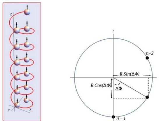
Fig 2: Schematic illustration of a single stranded helical molecules
