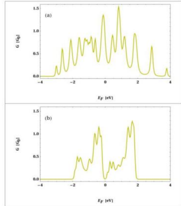
Fig 3: Electrical Conductance (measured in unit of G_0 ) as a function of Fermi Energy ( E_F ) for a long-range hopping (LRH) magnetic helix in (a) absence and (b) presence of light. Here, we set N = 10 and A_0 = 0.5 .
