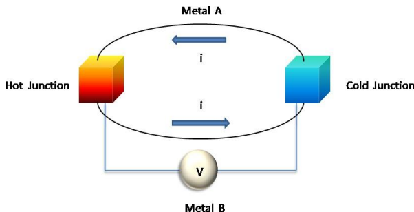
Fig 1: Schematic diagram of Seebeck effect where a thermal gradient induces a voltage drop at two junctions.
