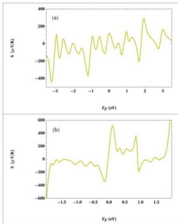
Fig 4: Seebeck coefficient (thermopower S ) as a function of Fermi Energy ( E_F ) for a long-range hopping (LRH) magnetic helix in (a) absence and (b) presence of light. Here, we set N = 10 and A_0 = 0.5 .
