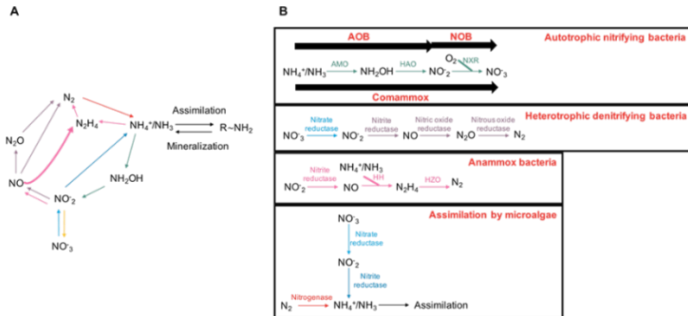
Fig. 2: The Nitrogen Cycle's main biological enzyme process that changes nitrogen into its many oxidation forms. Source: https://doi.org/10.1016/j.cub.2015.12.021 .
