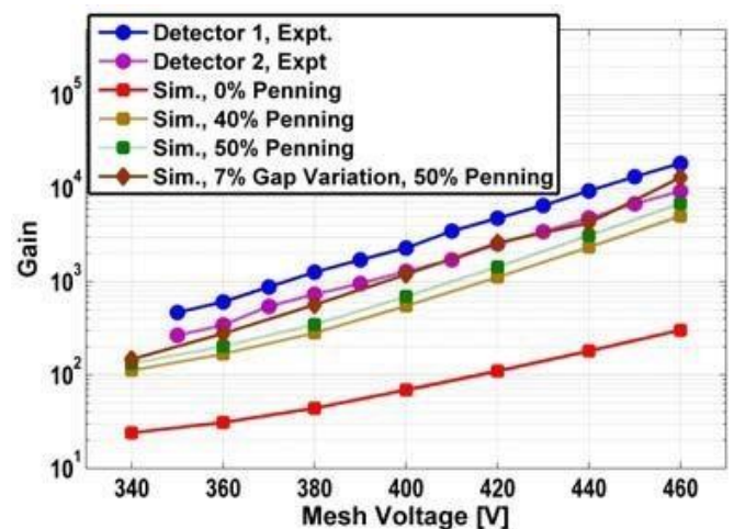
Fig. 3: Comparison of experimental gain with simulation in argon-isobutane (90:10) gas mixture for two bulk Micromegas detectors having amplification gap of 128Qm and pitch of 63 Qm.
