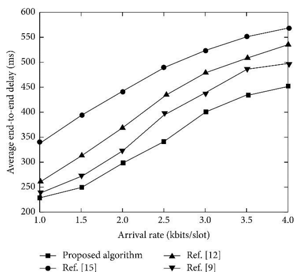
Fig. 3: Comparison of average end-to-end delay of different algorithms
